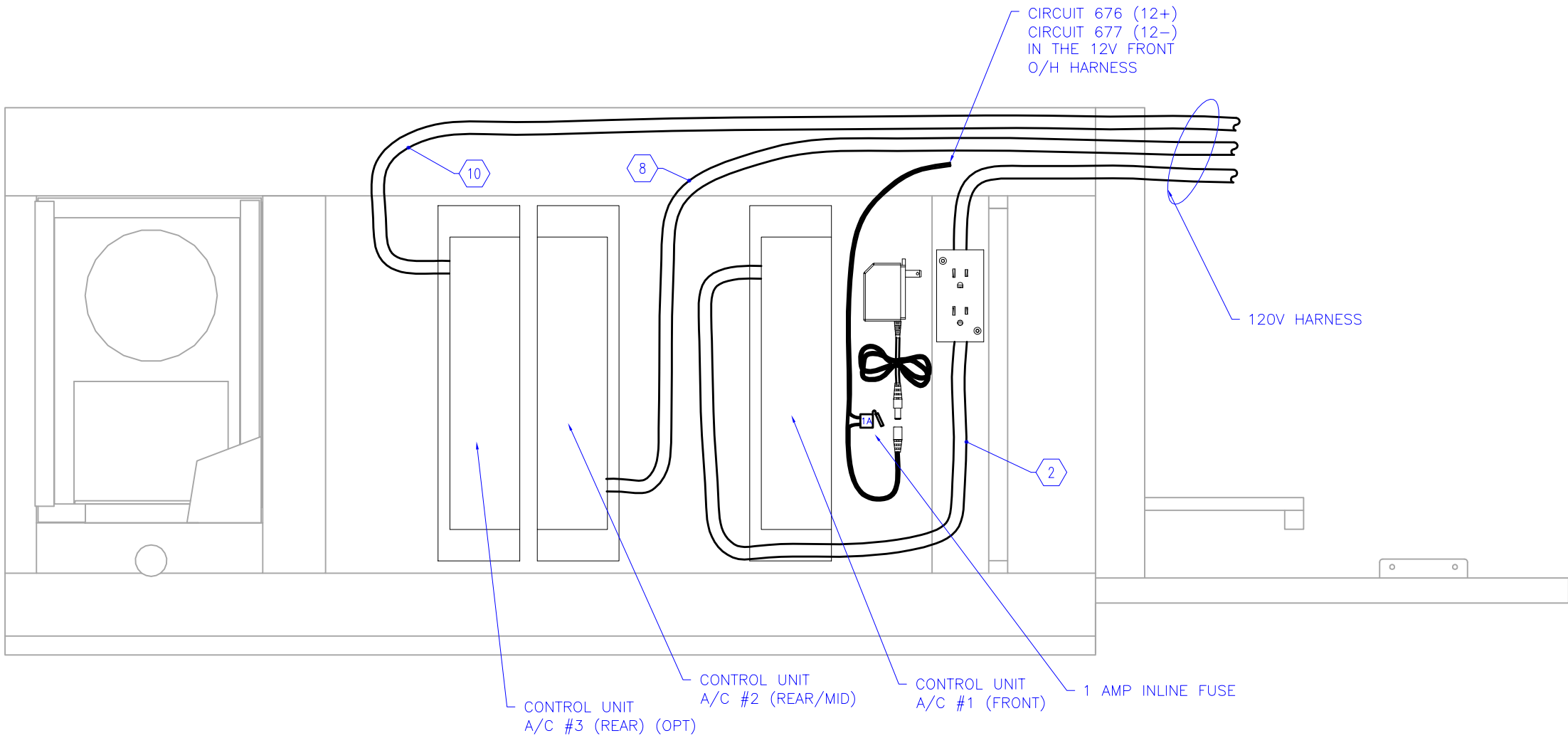
AUTO GEN TRANSFORMER AND RECEPT LOCATION
